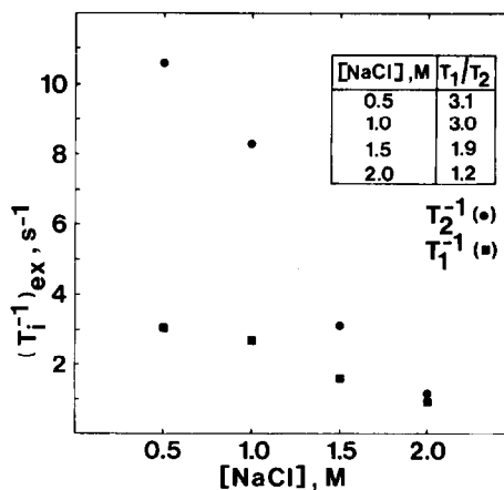
Fig.2. The effect of increasing NaCl concentration on ^{23}\text{Na} excess relaxation rates in the chromatin/NaCl system at a higher DNA concentration. The relaxation rates are normalised to a DNA concentration of 5.6 mM in phosphate ( A_{260} = 37 ). Results obtained with a different chromatin preparation to that in fig.1: (■) (T_1^{-1})_{\text{ex}} ; (●) (T_2^{-1})_{\text{ex}} .
